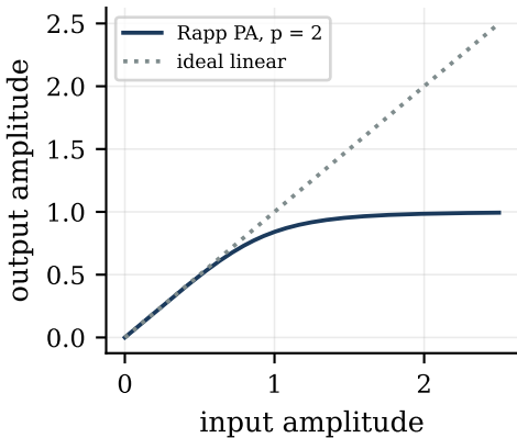
AM/AM characteristic
