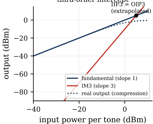
third-order intercept
