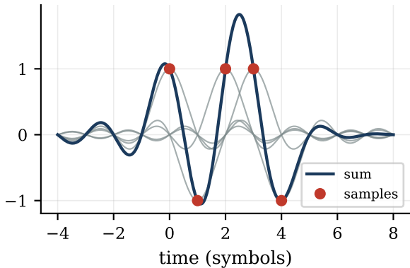
sinc (ideal Nyquist)
