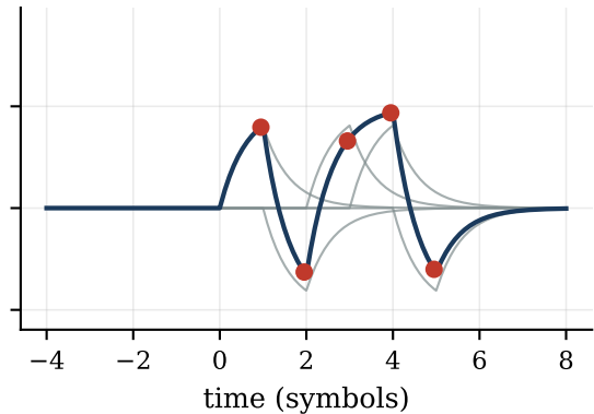
rectangular pulse through RC low-pass
