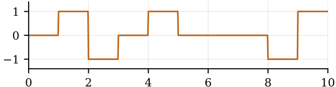
AMI / bipolar (T1)
