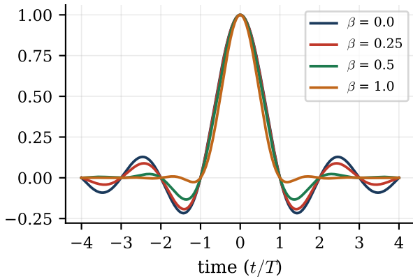
Impulse response
