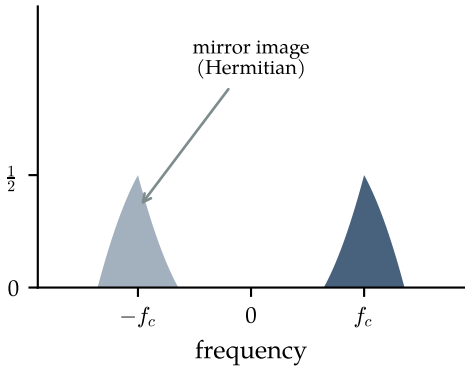
real bandpass signal x(t) : |X(f)|
