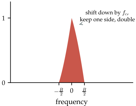
complex envelope \tilde{x}(t) : |\tilde{X}(f)|
