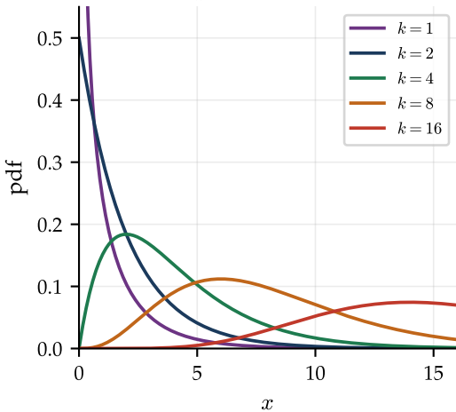
Central \chi_k^2 (unit-variance terms)
