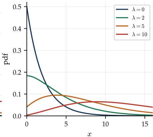
Noncentral \chi_2'^2(\lambda) : energy detector output
