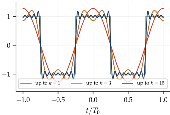
partial Fourier sums of a square wave
