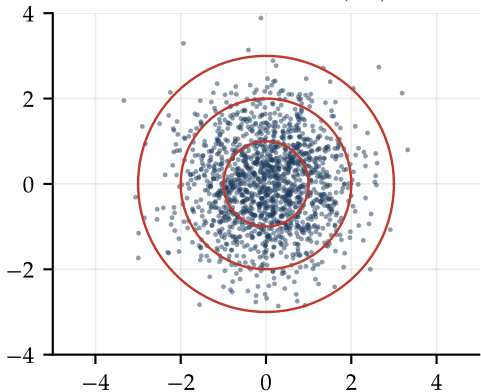
whitened: \mathbf{L}^{-1}\mathbf{x} \sim \mathcal{N}(\mathbf{0}, \mathbf{I})
