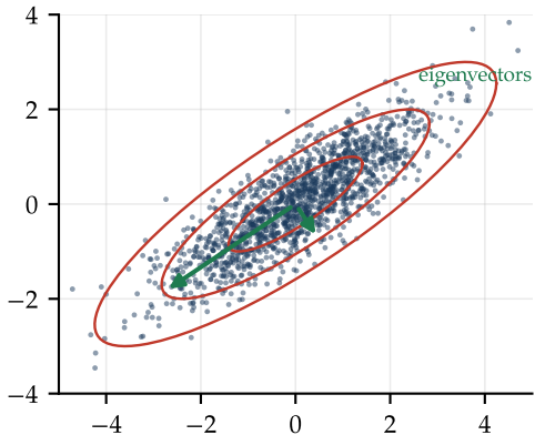
correlated: \mathbf{x} = \mathbf{L}\mathbf{w} , \mathbf{C} = \mathbf{L}\mathbf{L}^T
