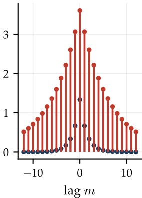
AR(1): R_x[m]
