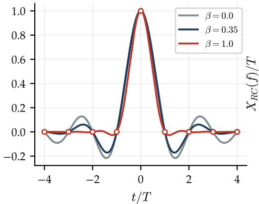
RC pulse: zero ISI at t = nT
