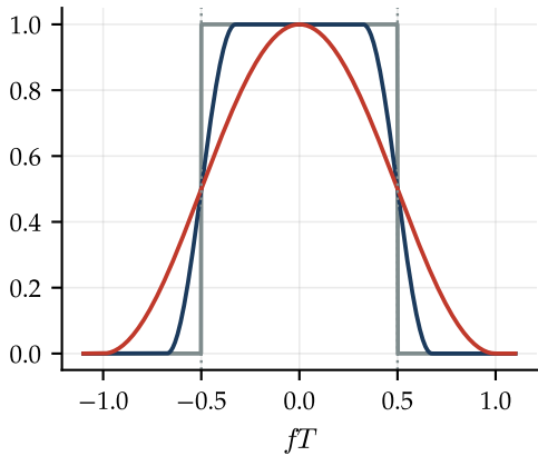
spectrum: odd symmetry about 1/2T
