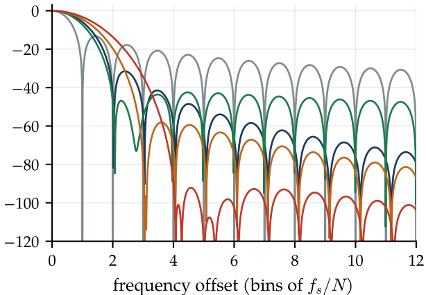
spectra: wider main lobe buys lower sidelobes
