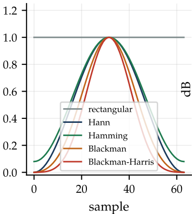
time shapes ( N = 64 )
