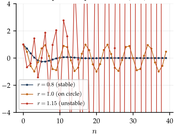
impulse response r^n \cos(\omega_0 n)
