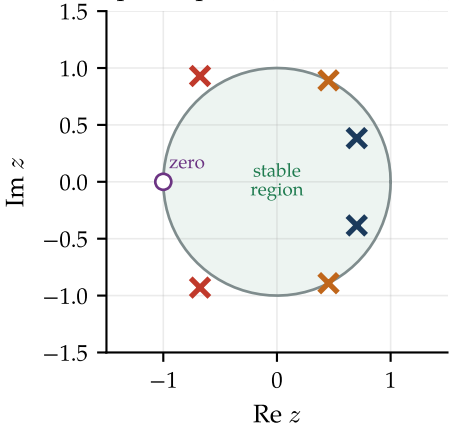
z -plane: poles (x) and zero (o)
