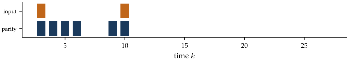
recursive encoder, two 1s seven apart: back to zero (parity weight 6)
