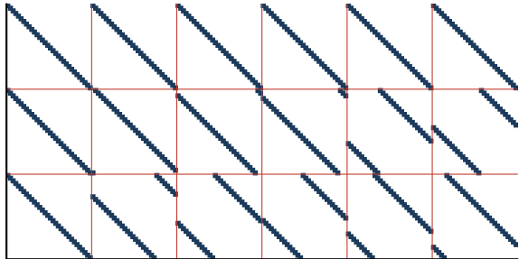
quasi-cyclic, Z = 32 : 18 shifted identities
