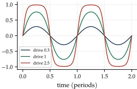
y = \tanh(x) : big inputs flatten into squares
