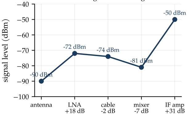
A level diagram: add the gains
