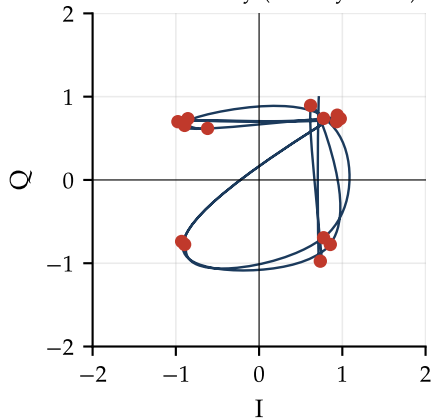
highway frame: complex envelope wanders slowly (dots: symbols)
