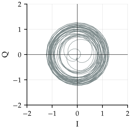
Earth frame: analytic signal whirls round at f_c
