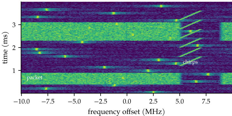
A synthetic waterfall: hops, packets and chirps
