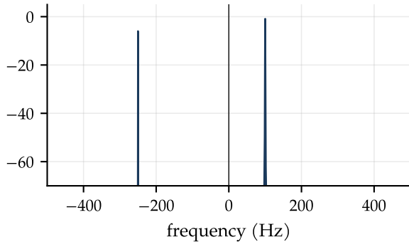
complex (I and Q): +100 and -250 Hz are distinct
