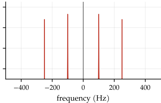
real part only: every tone gets a mirror
