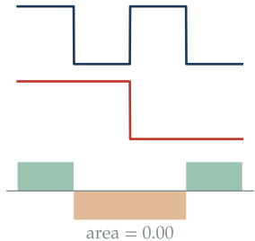
Walsh codes
