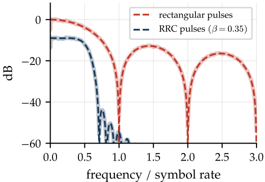
Simulated PSD (solid) vs |P(f)|^2 (dashed)
