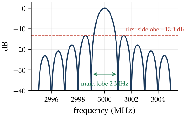
A 1 \mu s burst of 3 GHz carrier
