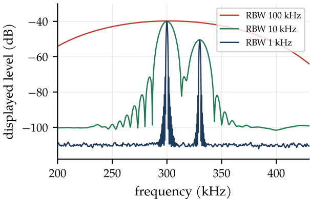
Narrower RBW: lower floor, finer detail
