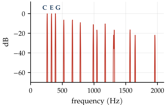
Spectrum view: three notes and their overtones
