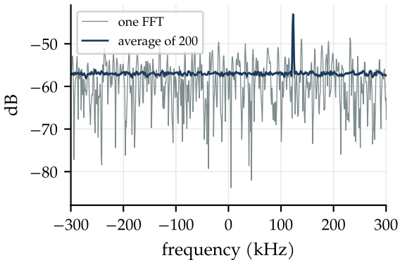
A weak spur emerges from averaged noise
