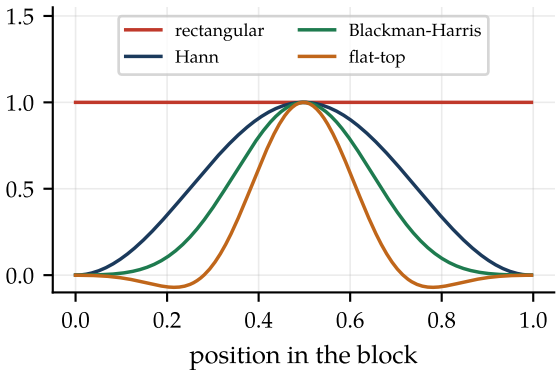
Four windows: how fast the frame fades out
