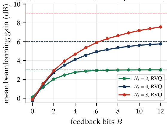
(b) limited feedback (dashed: perfect CSIT)
