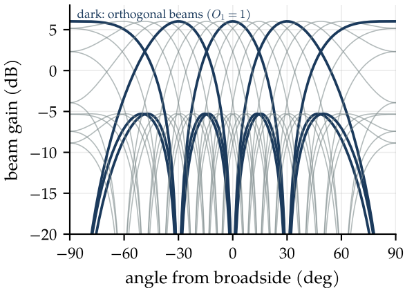
(a) DFT codebook, N_1 = 4 , O_1 = 4
