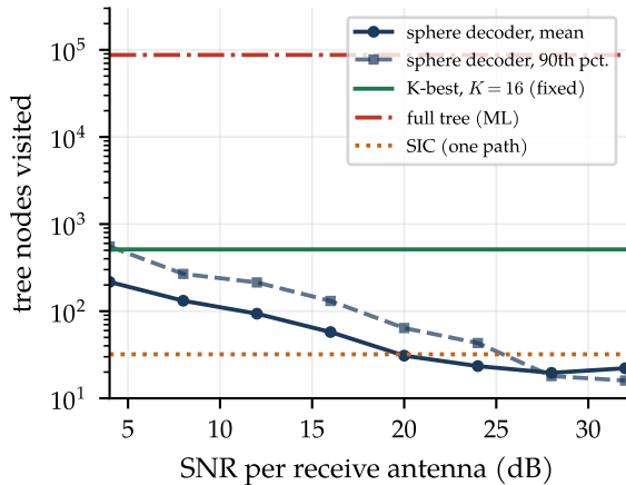
(b) complexity, 4 \times 4 16-QAM
