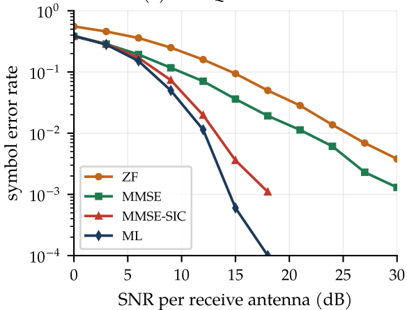
(a) 4 \times 4 QPSK detectors
