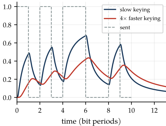
Pulses smear into each other (ISI)
