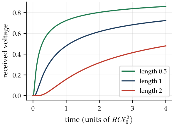
Step response: delay grows as \text{length}^2
