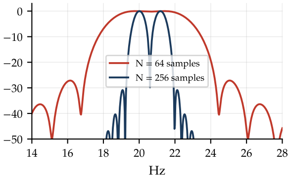
Resolution needs observation time
