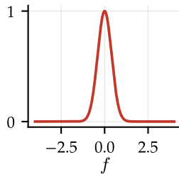
Gaussian
