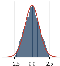
sum of 2 uniforms
