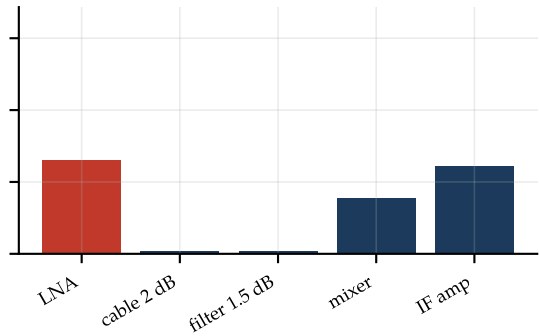
LNA at the antenna (mast-head) cascade NF = 2.23 dB
