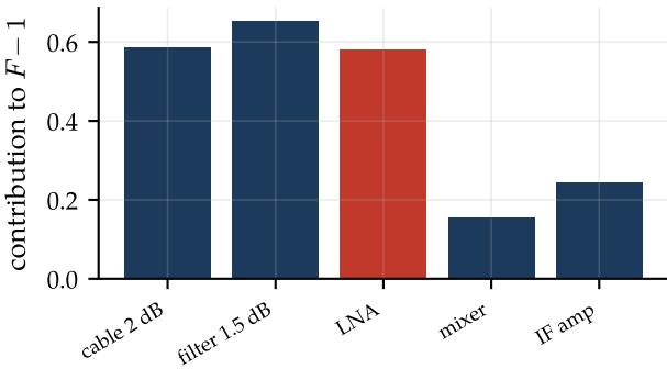
LNA after cable and filter cascade NF = 5.07 dB
