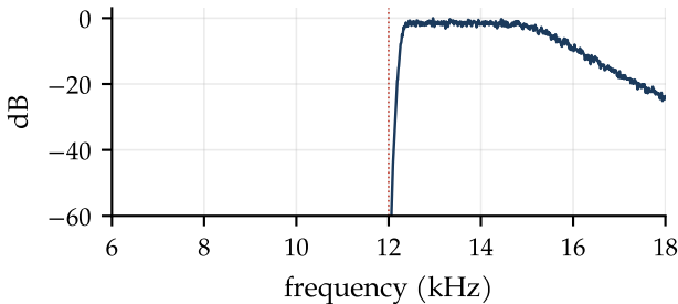
SSB, upper sideband
