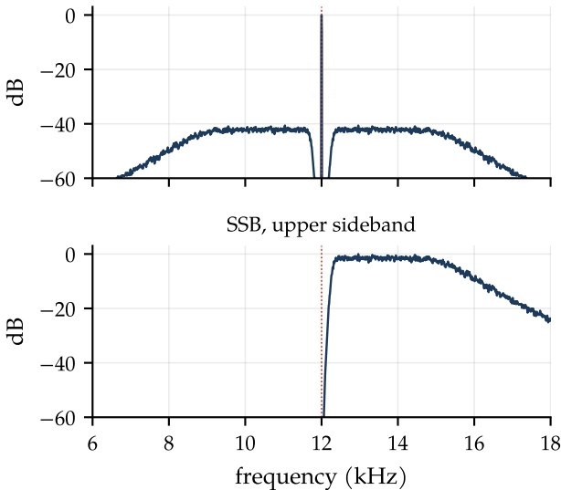
AM (DSB with carrier), \mu=0.8
