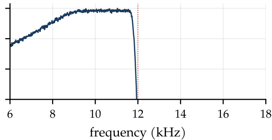
SSB, lower sideband
