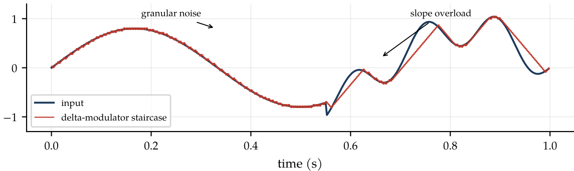
Delta modulation: one bit per sample, fixed step
