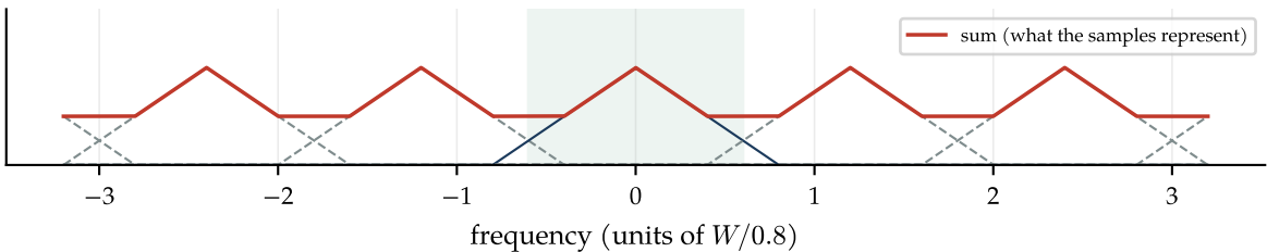
sampled at f_s = 1.5W : replicas overlap (aliasing)
