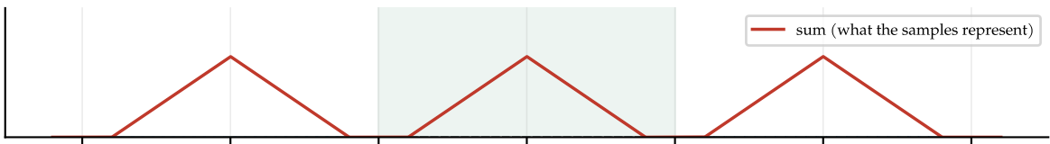
sampled at f_s = 2.5W : replicas separate
