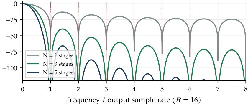
CIC decimator response: nulls fall on the alias bands
