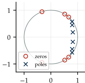
elliptic pole-zero
