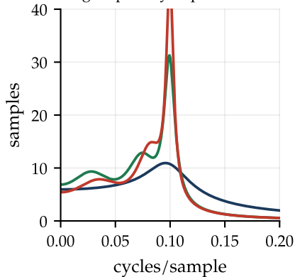
group delay in passband
