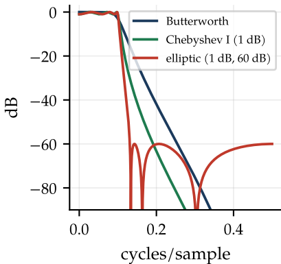
6th-order IIR magnitude
