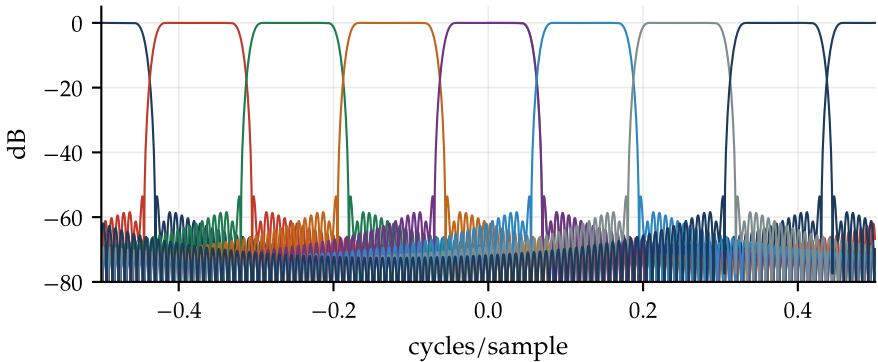
8-channel polyphase filter bank (channelizer)
