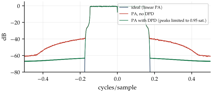
Digital predistortion at 10 dB back-off
