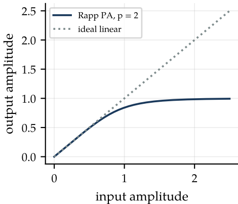
AM/AM characteristic
