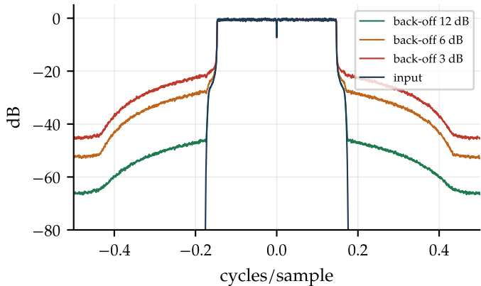
OFDM spectral regrowth versus PA back-off
