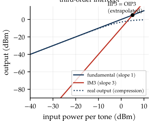
third-order intercept
