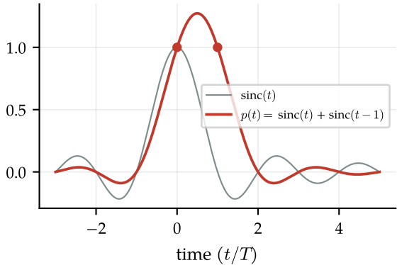
Duobinary pulse: controlled ISI
