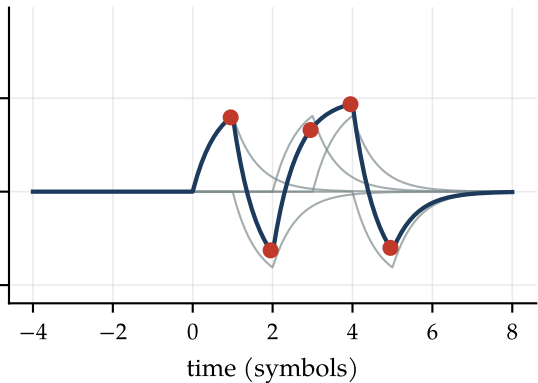
rectangular pulse through RC low-pass
