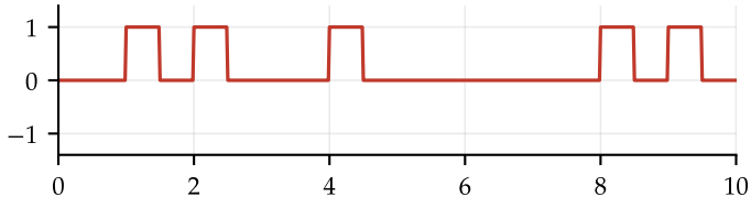
Manchester (10BASE-T)
