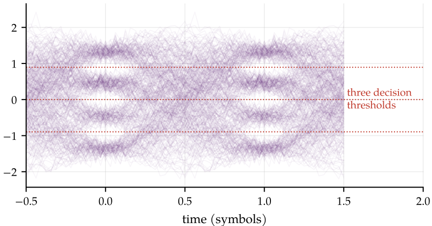
PAM-4 eye (as in 400G Ethernet, PCIe 6.0, GDDR6X)
