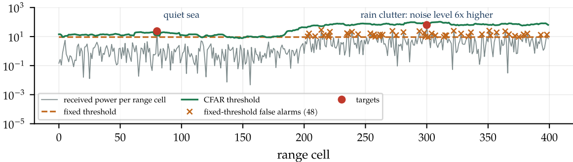
Constant false-alarm rate: let the threshold follow the noise
