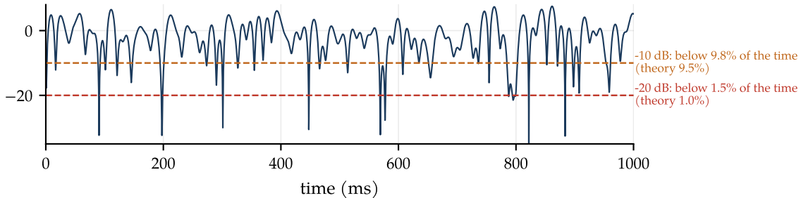
Rayleigh fading: the exponential power law in action (40 Hz Doppler)
