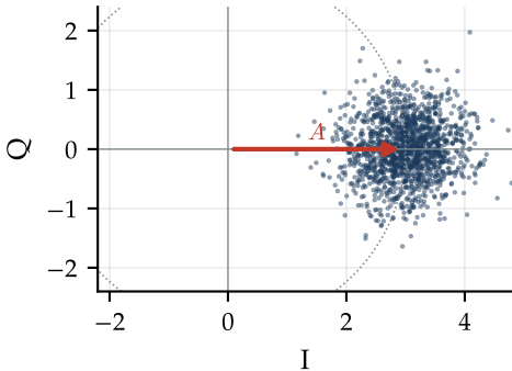
strong carrier: Rice, nearly Gaussian
