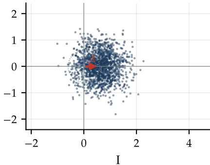
weak carrier: noise takes over
